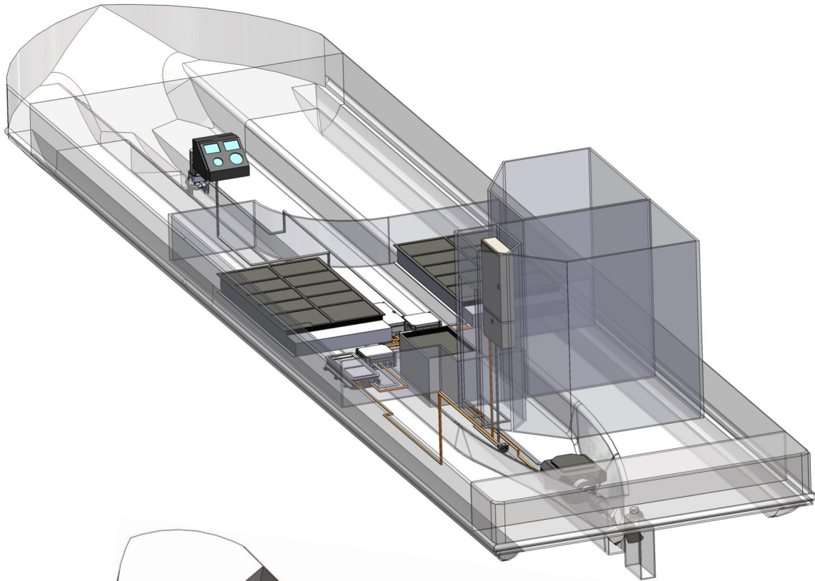
Figure A4.5: Powertrain layout within retrofit vessel and enclosing superstructure
