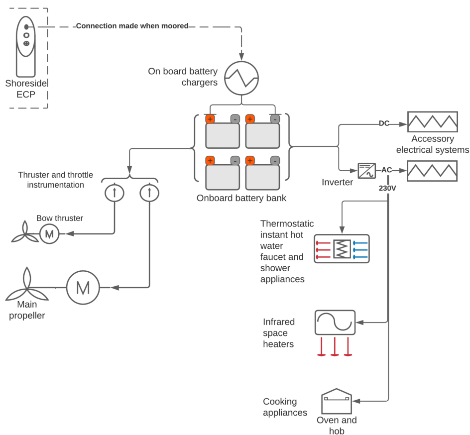
Figure 7.7: Schematic showing principal electrical systems replacing fossil fuel dependent systems
