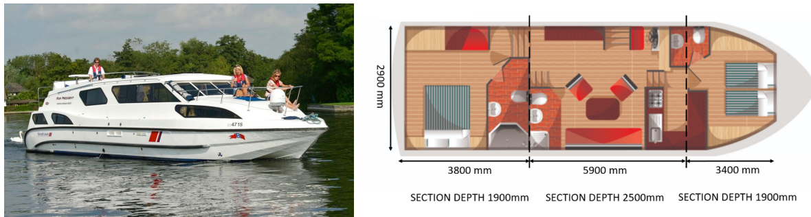
Figure 5.3: A President class hire vessel and dimensions
