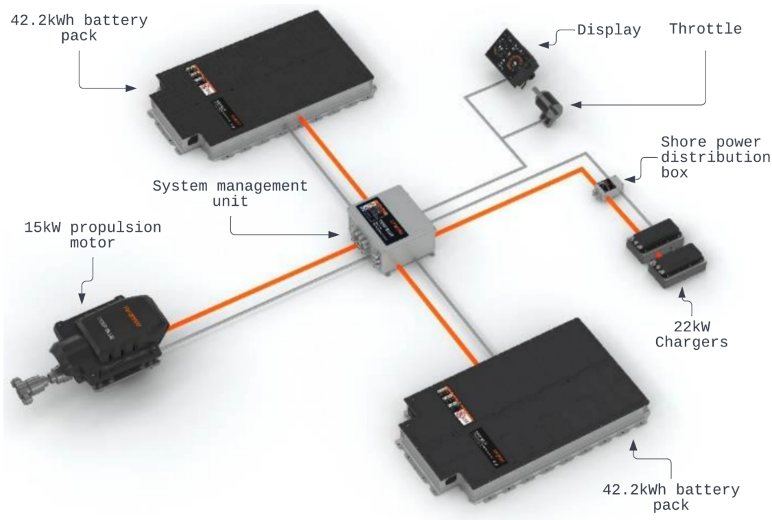
Figure 5.4: Powertrain overview 6
