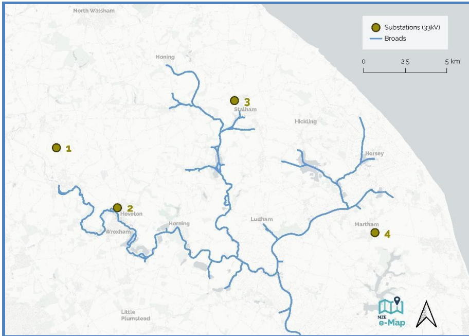
Figure A5.4: 33kV substations and headroom estimates
