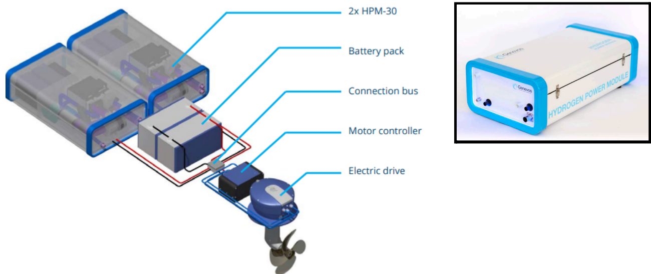
Example: Vessel powertrain with 56 kW HPM propulsion
